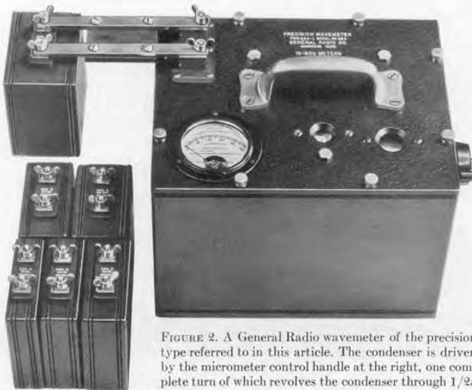
FIGURE 2. A General Radio wavemeter of the precision type referred to in this article. The condenser is driven by the micrometer control handle at the right, one complete turn of which revolves the condenser through 1/25 of a semicircle. The micrometer shaft carries an accurate
