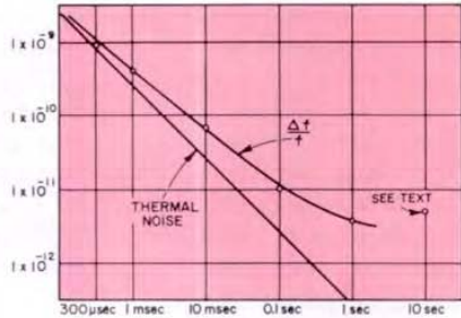
Figure 2. Theoretical and measured stability of a crystal oscillator.
