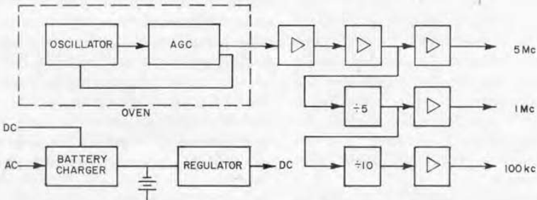
Figure 10. Block diagram of Standard Frequency-Oscillator.
