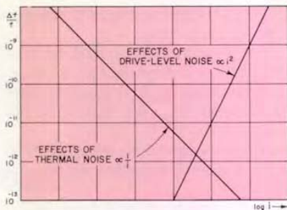
Figure 4. Effects of crystal current on short-term stability.
