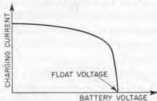
Figure 17. Battery recharge characteristic.
