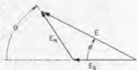
Figure 5. Vector diagram showing phase shift due to stray coupling to output.
