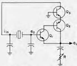
Figure 12. Basic oscillator circuit.
