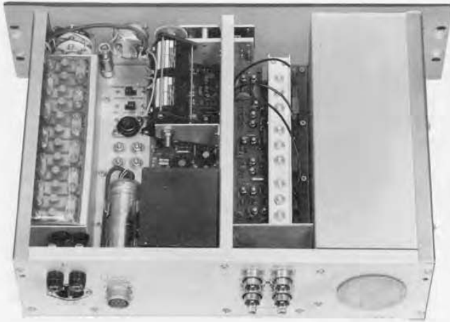
Figure 9. View of oscillator with cover removed.
