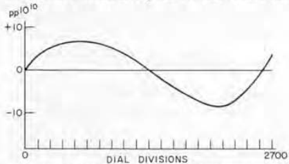
Figure 15. Tracking error of varactor tuning.
