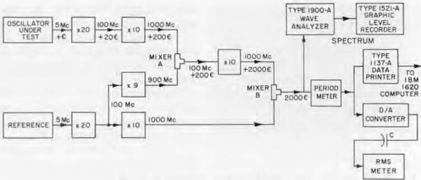
Figure 18. Block diagram of measuring system.
