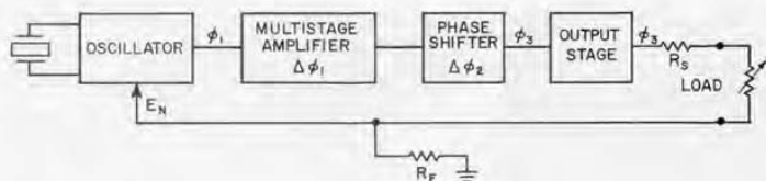
Figure 6. Typical block diagram for a precision oscillator.
