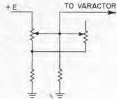
Figure 14. Linearizing network for varactor.
