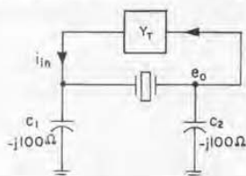
Figure 11. Basic oscillator network.
