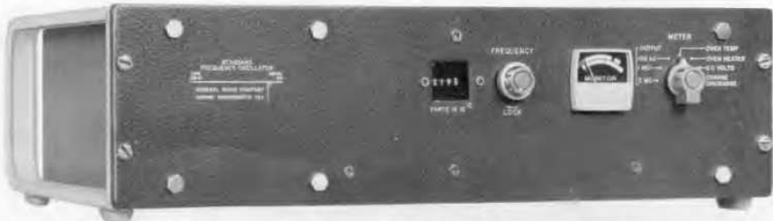
Figure 8. Panel view of Type 1115-B Standard-Frequency Oscillator.
