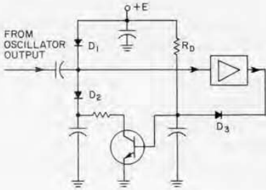
Figure 13. Basic AGC circuit.
