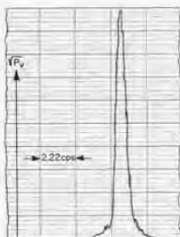
Figure 22. Center portion of spectrum of Figure 21, measured with 0.54-cycle bandwidth. Vertical scale is linear ( \sqrt{\text{power}} ).
