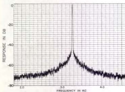
Figure 21. X-band power spectrum of two Type 1115-B Standard-Frequency Oscillators. Analyzer bandwidth is 10 cps.
