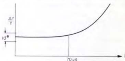
Figure 3. Drive-level sensitivity of 5-Mc crystal. 6
