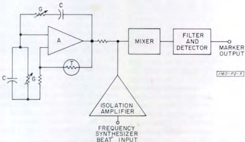
Figure 3. Diagram of marker-generator section.
