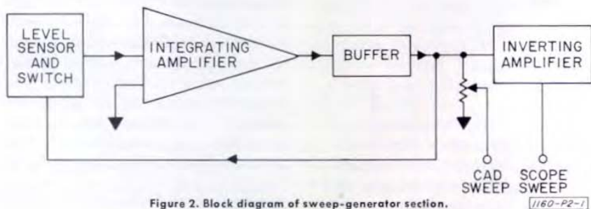
Figure 2. Block diagram of sweep-generator section.
