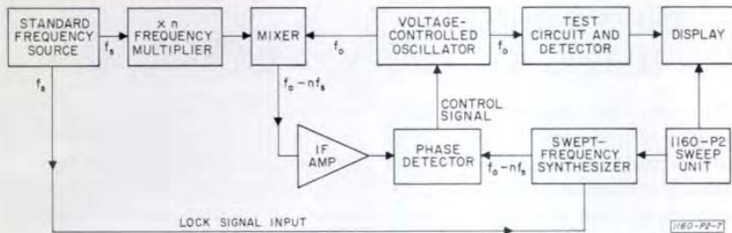
Figure 9. Block diagram of a frequency-conversion system.
