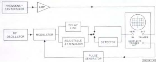
Figure 3. Equipment setup for measurement of delay line.
