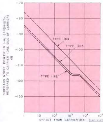
Figure 2. Phase-noise power-density distribution in GR 1160-series synthesizers.
