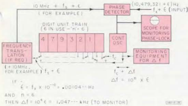
Figure 2. Block diagram illustrating frequency-tracking scheme. \epsilon represents any small frequency drift of the unknown, which is matched and canceled by the servo loop.
