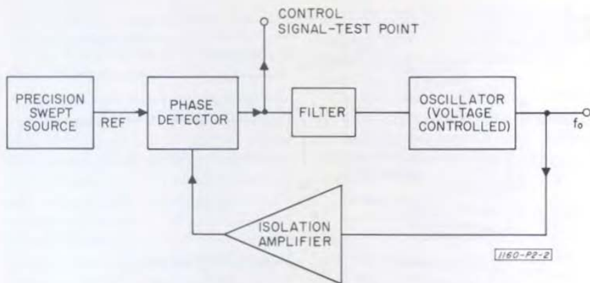
Figure 7. Setup for swept-frequency evaluation of phase-locked loop.
