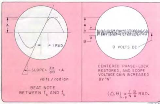
Figure 9. Oscilloscope calibration for phase noise.
