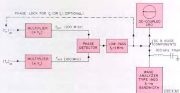
Figure 1. Equipment setup for the measurement of phase-noise density.
