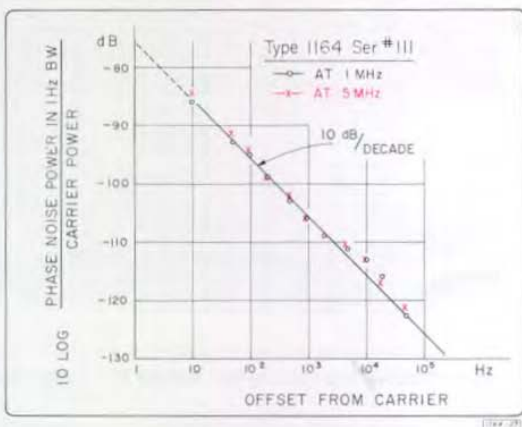
Figure 10. Single-side phase-noise power-density, referred to carrier.
